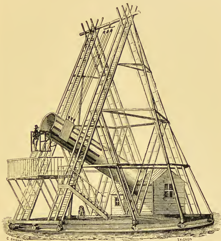
FIG. 83.—Herschel's 40-foot telescope.
